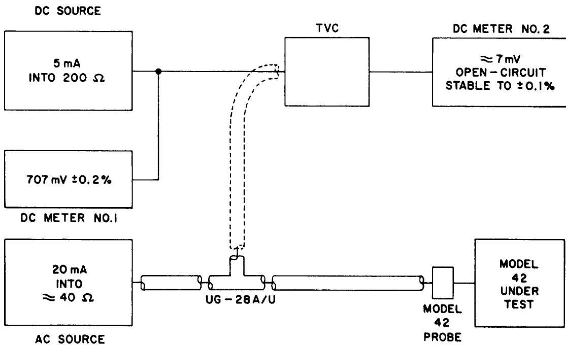
Figure 10. Connections
